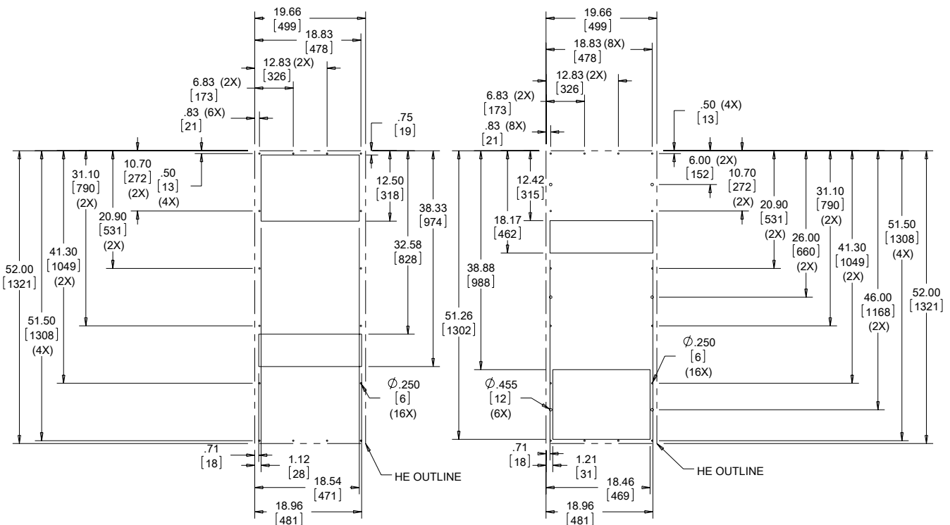
Cutout Dimensions (External Mount)
